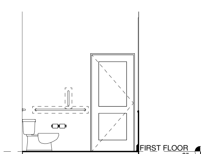
TOILET NORTH 1/4" = 1'-0"
