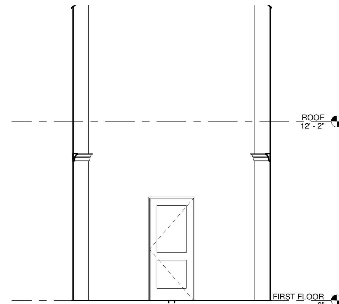
VESTIBULE WEST 1/4" = 1'-0"
