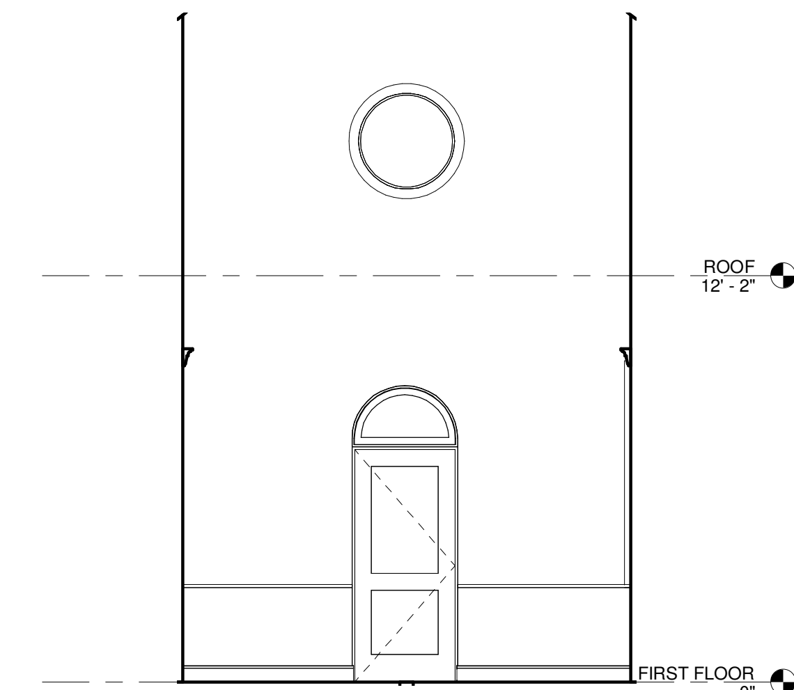
VESTIBULE EAST 1/4" = 1'-0"
