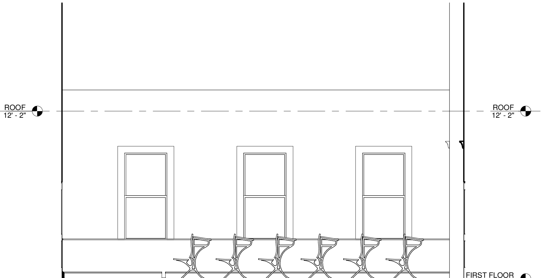
CLASSROOM NORTH 1/4" = 1'-0"
